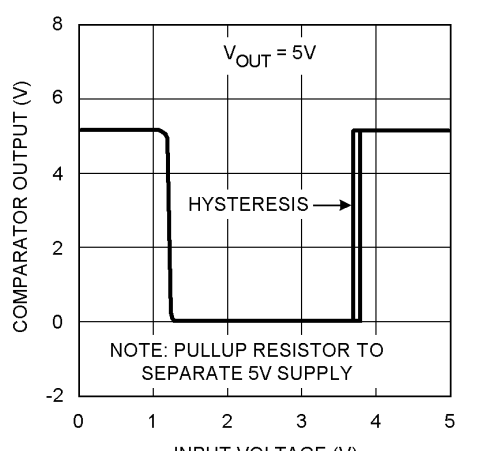
LP4951C Error Comparator Output
